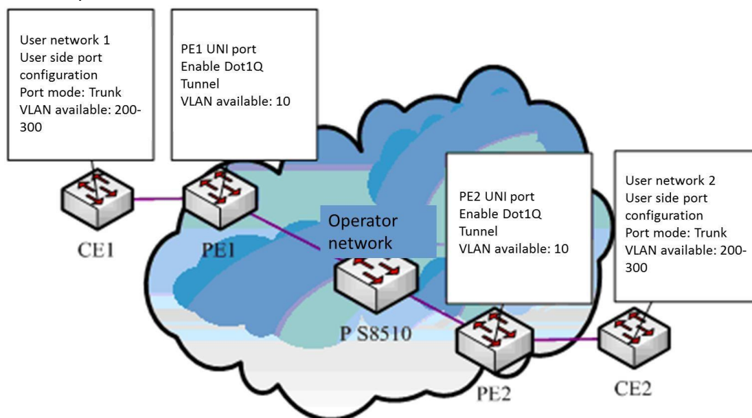
Figure 3 Typical configuration of Dot1Q tunnel
